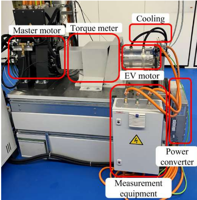
Fig. 2: Test bench provided for the study
